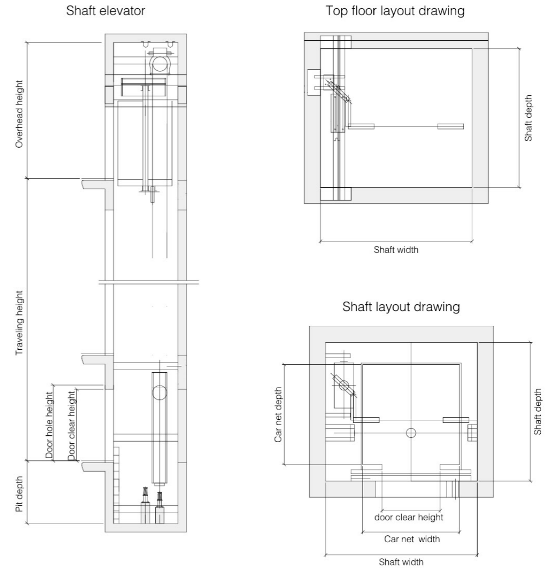
Machine roomless passenger elevator specifications
